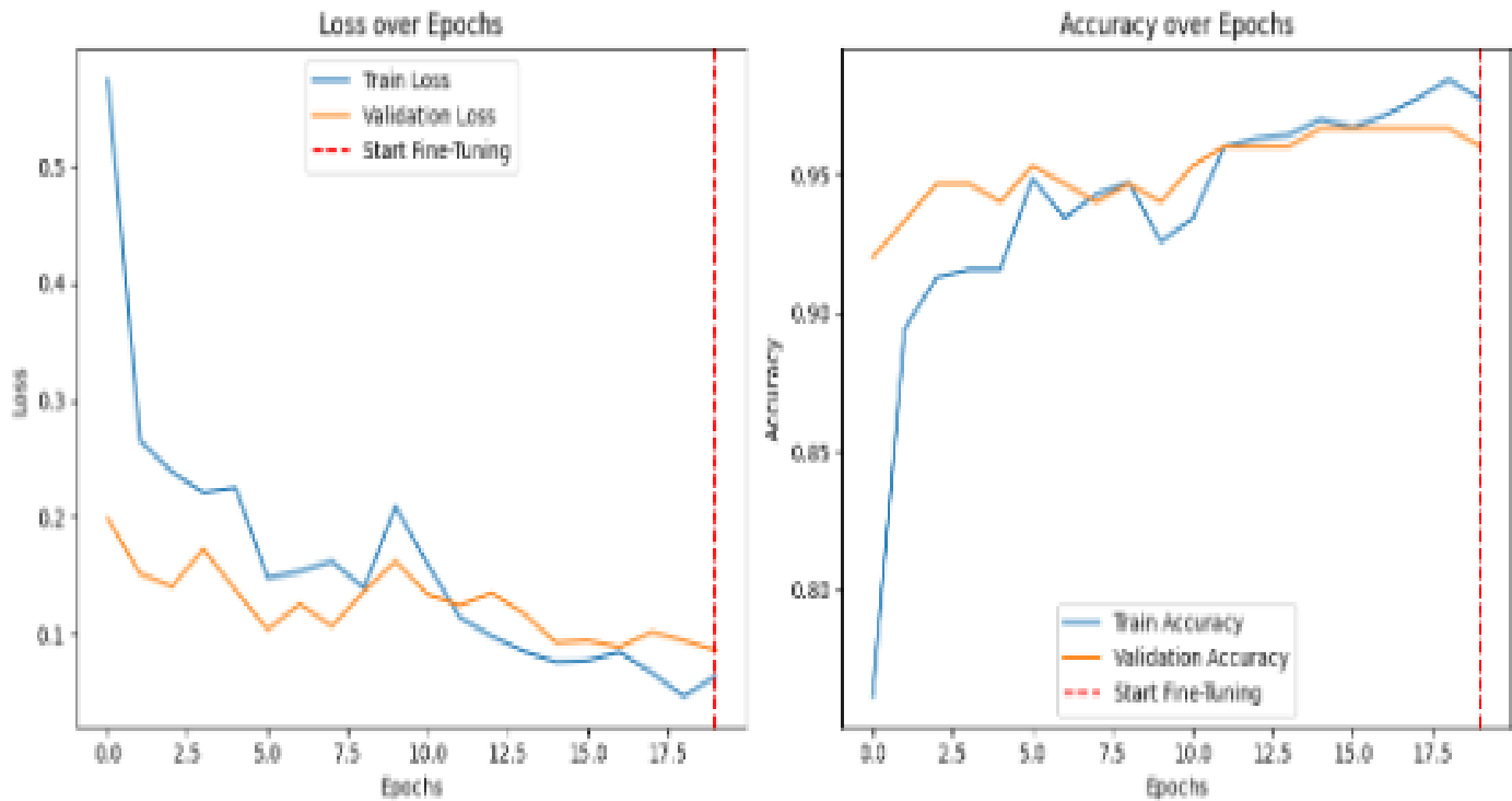
Figure: AlexNet Accuracy/Loss Plot
