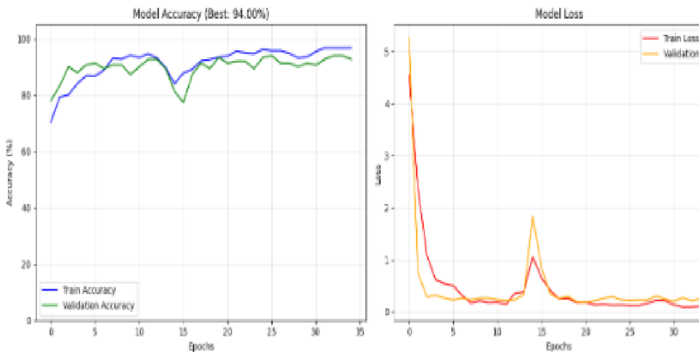
Figure: Custom CNN Training Curves
